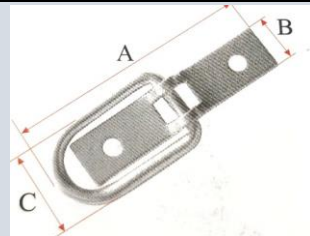
GH-15 ZINC 81X16X30 PRS004
