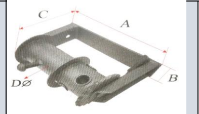
TT-60 C/C 250X50X150X60 PRS038
